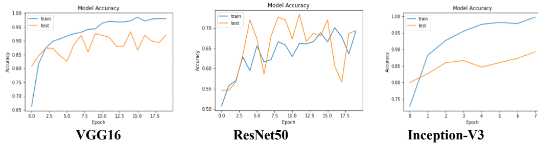
Figure 1. VGG16, ResNet50 and Inception-V3 Networks Accuracy Plots
